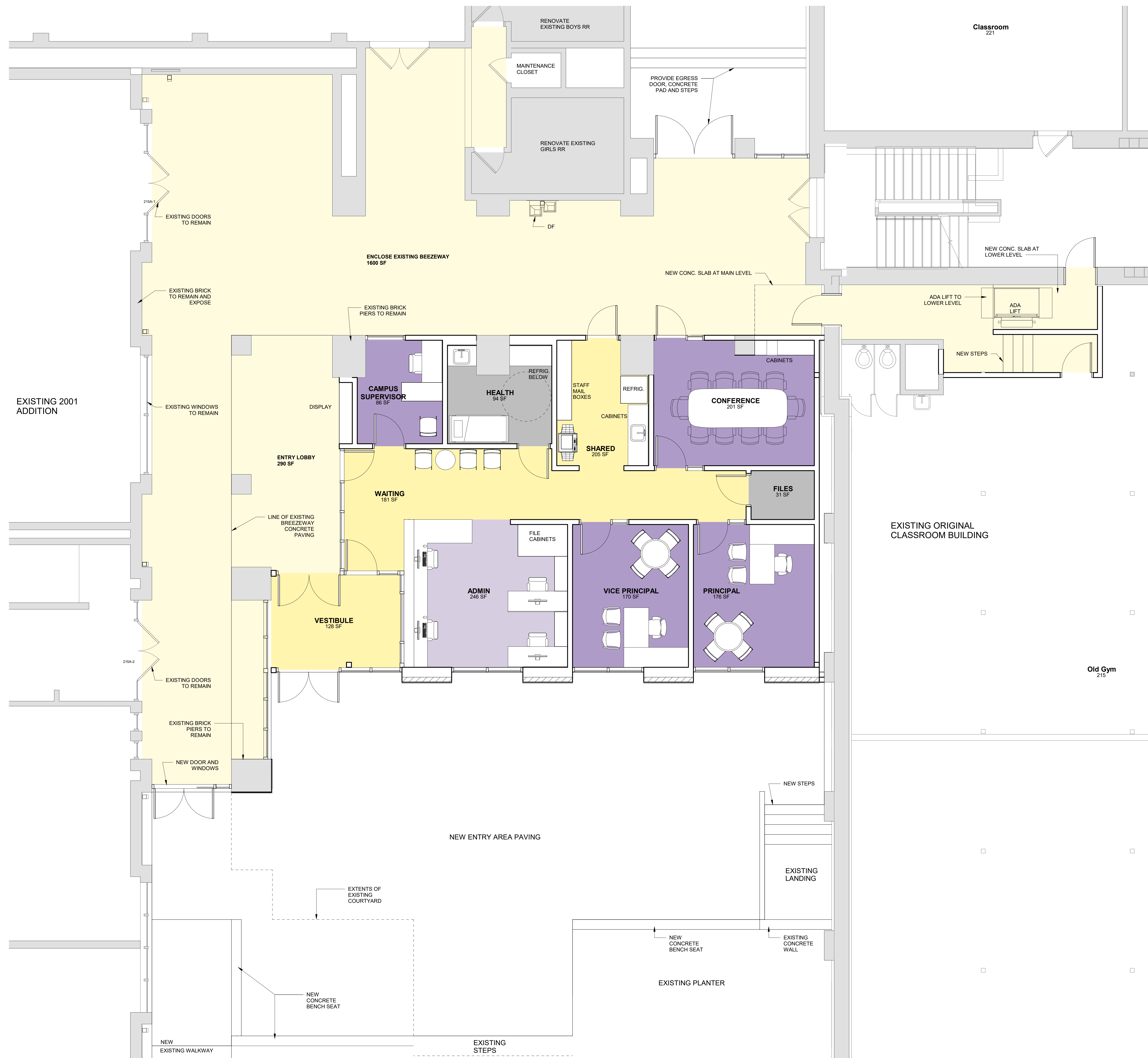
FLOOR PLAN - 1/4" = 1'-0"
